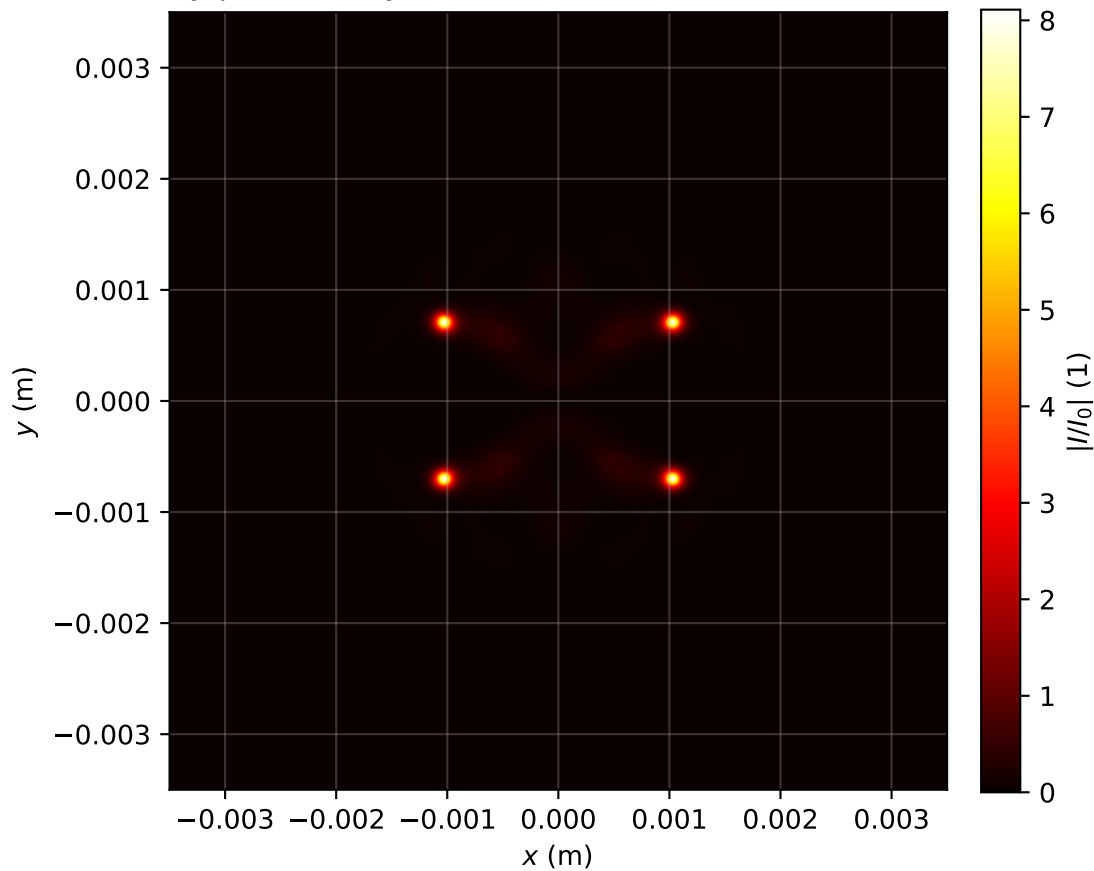
Intensity profile I(x, y, z = 1.831)/I_0 , P_{in}=9.0P_{cr} , artificial time
